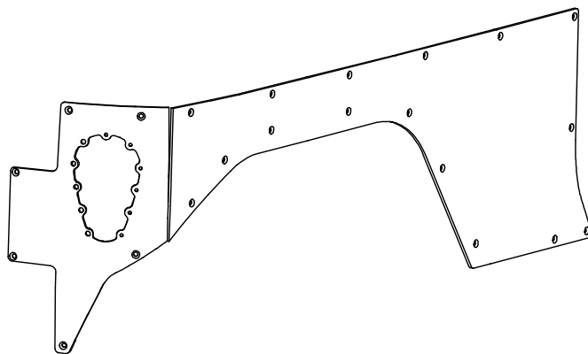
MB1138-W02 QTY 1
