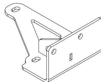
MB1227-YJ-07 Qty 1
