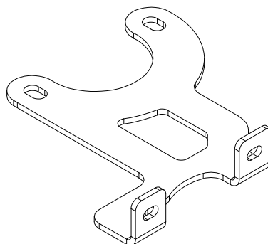
MB1227-TJ-07 Qty 1
