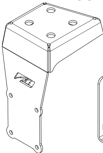
MB3032-2-05 Qty 1
