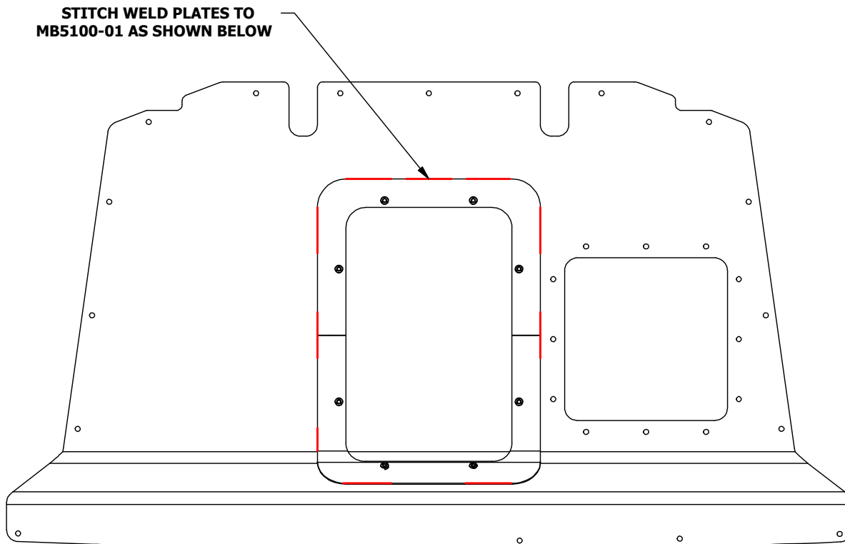
Bottom/Underside View
