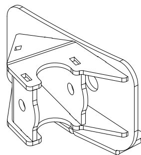
MB3029-W01 Qty 1
