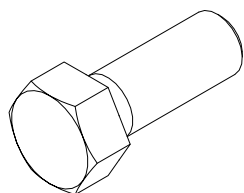
3/8\"-16 x 1\" Gr. 8 NC Hex Cap Screw, YZ Qty 8
