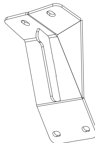
MB1267-W02 Qty 1
